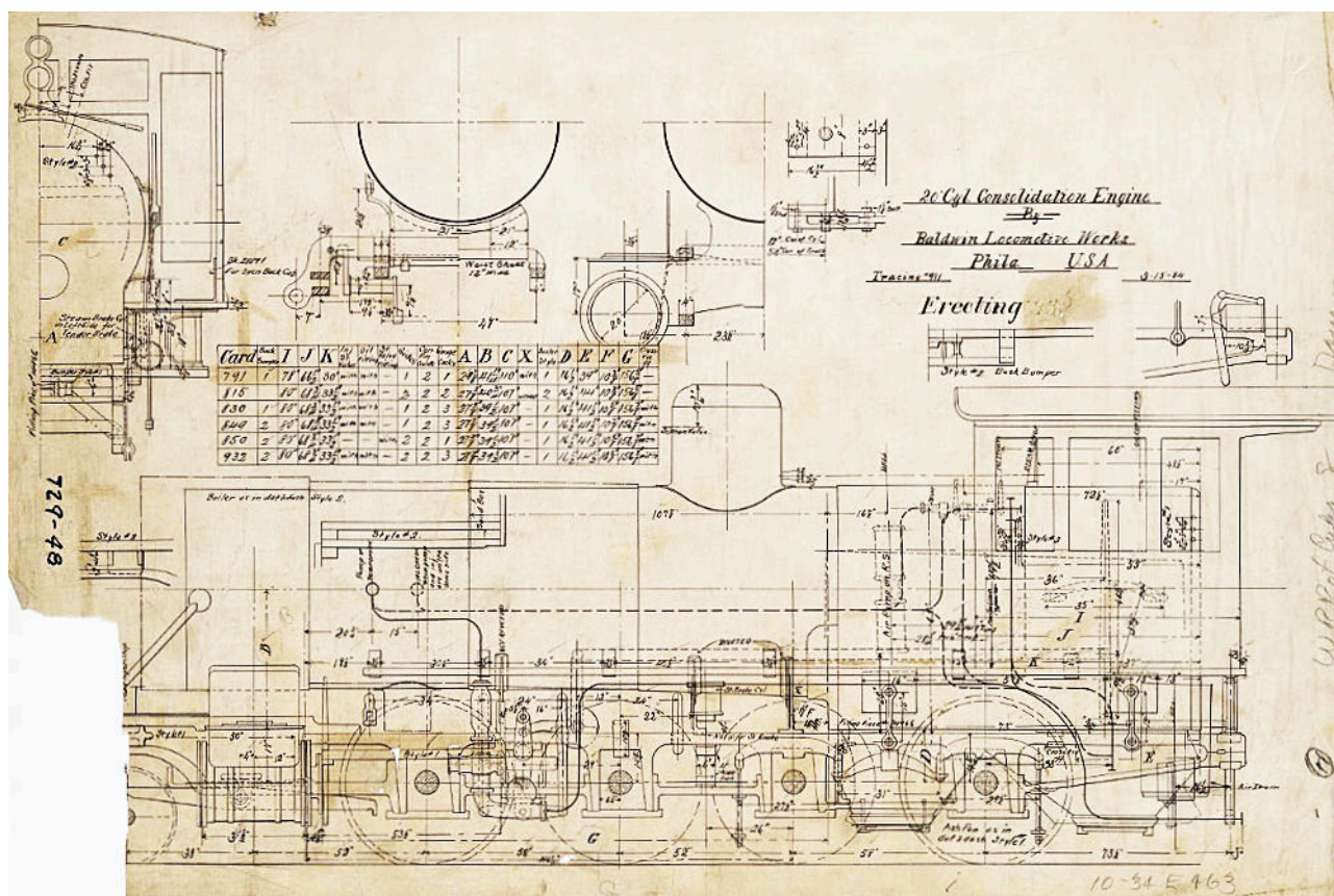
This Baldwin erecting card drawing from the DeGolyer Library collection shows FC Oeste no. 8 2 of 1884..
