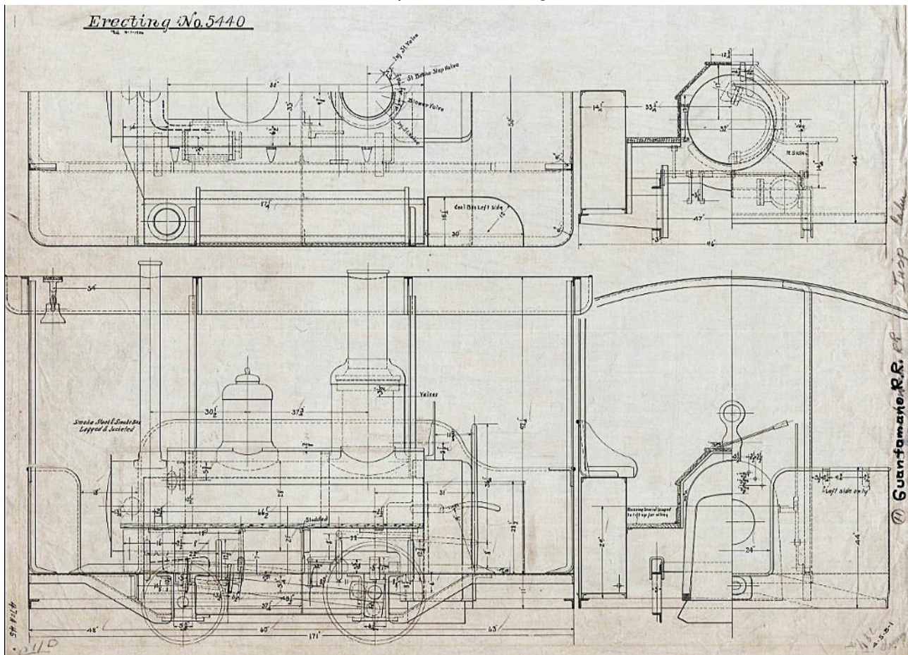
A Baldwin erecting card drawing of the GRR's 1906 inspection car. The drawing is from the DeGolyer Library's online archive. As with earlier Rogers inspection cars for Peru, the low and widely spaced side tanks doubled up as benches for inspectors or track gangs.
