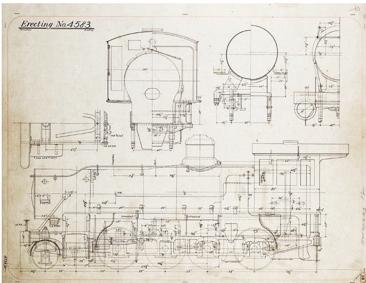
A Baldwin erecting card drawing for FC de Matanzas nos. 18 2 and 19 2 of 1900. Found in the De Golyer Library online archive. A very similar drawing is also in that collection showing locomotive 3 2 , the first of the class.
