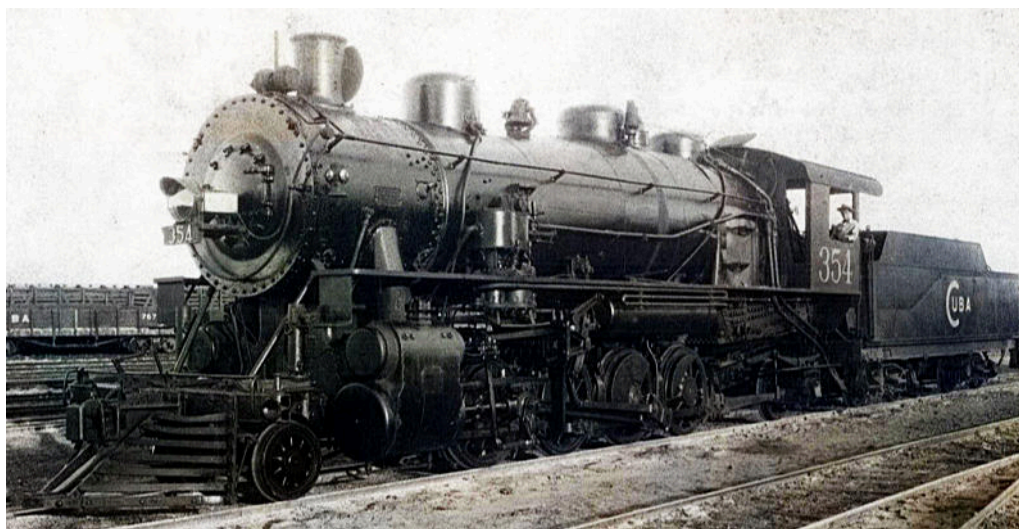
FC de Cuba no 350 ALCo publicity card details.
