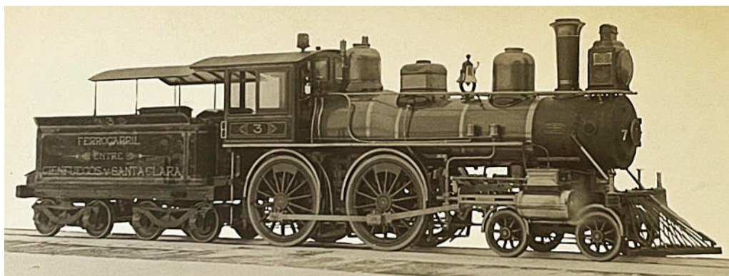
The railway's no. 3 1 built in 1853 by Rogers. The tender bears the later words 'Santa Clara' rather than the earlier version 'Villa Clara'.
